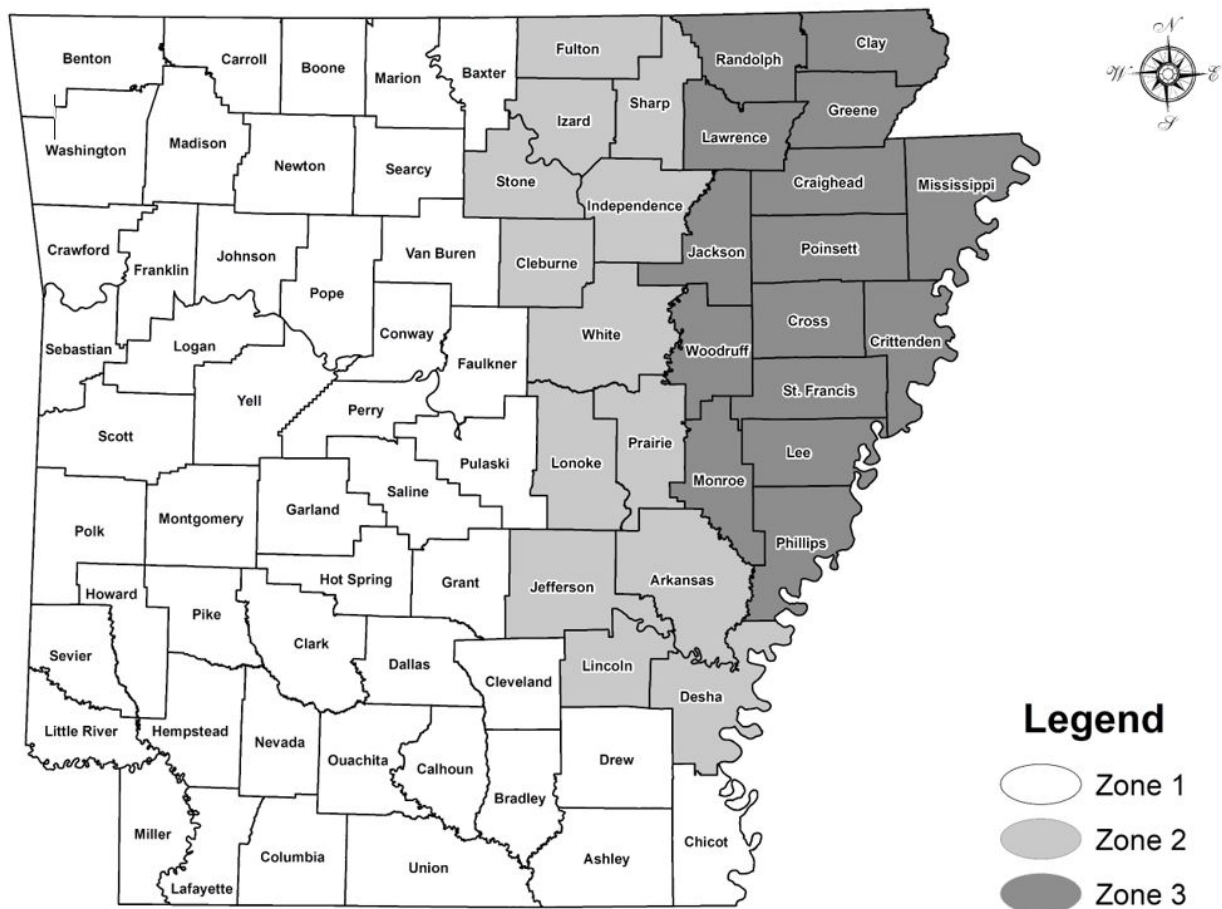
FIGURE 1 ARKANSAS SEISMIC ZONES
